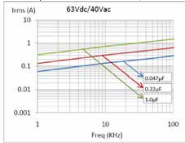
Max. Current (Irms) vs. Frequency (Sinusoidal Waveform at T \leq 55^\circ C )
