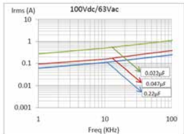
Max. Current (Irms) vs. Frequency (Sinusoidal Waveform at T \leq 85^\circ \text{C} )
