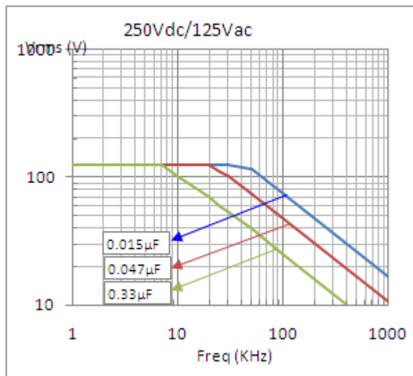
Max. Voltage (Vrms) vs. Frequency (Sinusoidal Waveform at T \leq 85^\circ C )
