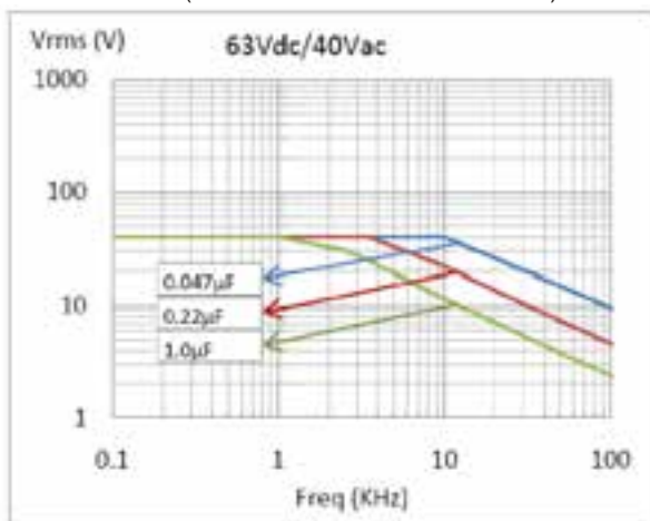
Max. Voltage (Vrms) vs. Frequency (Sinusoidal Waveform at T \leq 55^\circ C )
