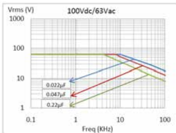
Max. Voltage (Vrms) vs. Frequency (Sinusoidal Waveform at T \leq 85^\circ \text{C} )
