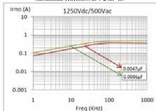
Max. Current (Irms) vs. Frequency (Sinusoidal Waveform at T \leq 85^\circ C )
