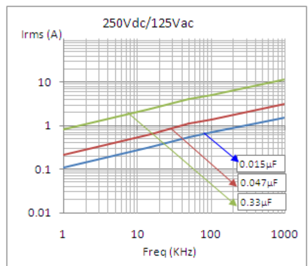
Max. Current (Irms) vs. Frequency (Sinusoidal Waveform at T \leq 85^\circ C )
