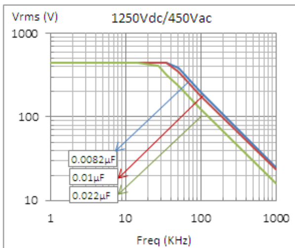
Max. Voltage (Vrms) vs. Frequency (Sinusoidal Waveform at T ≤ 85° C)
